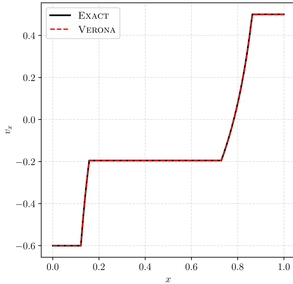
Shock Tube II
